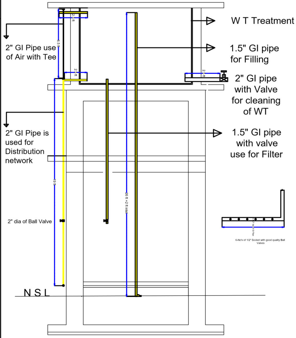
Detail of sanitary Work
