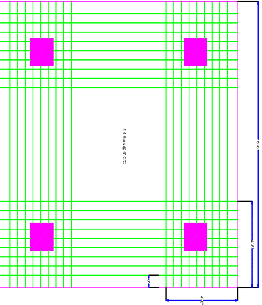
Foundation Reinforcement Plan
