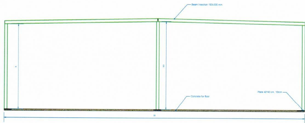
steel Structure details
