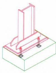
steel column and concrete column details
