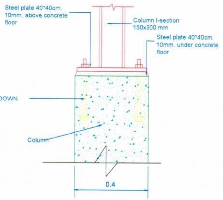
steel column and concrete column details
